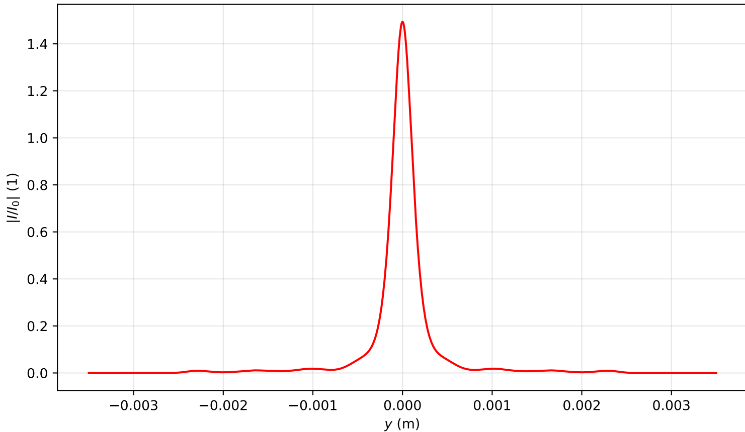
Intensity profile I(x=0, y, z=3.981)/I_0 , P_{in}=3.0P_{cr} , artificial time
